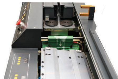
In-line notching, glue application, and nipping station
